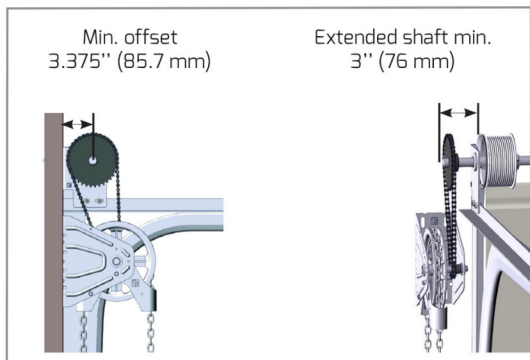
Chain hoist may be mounted on either side of the door
