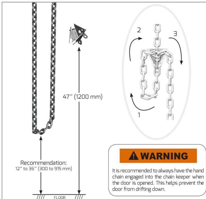
Chain hoist may be mounted on either side of the door
